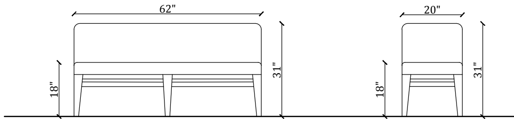
BENCH FRONT VIEW
